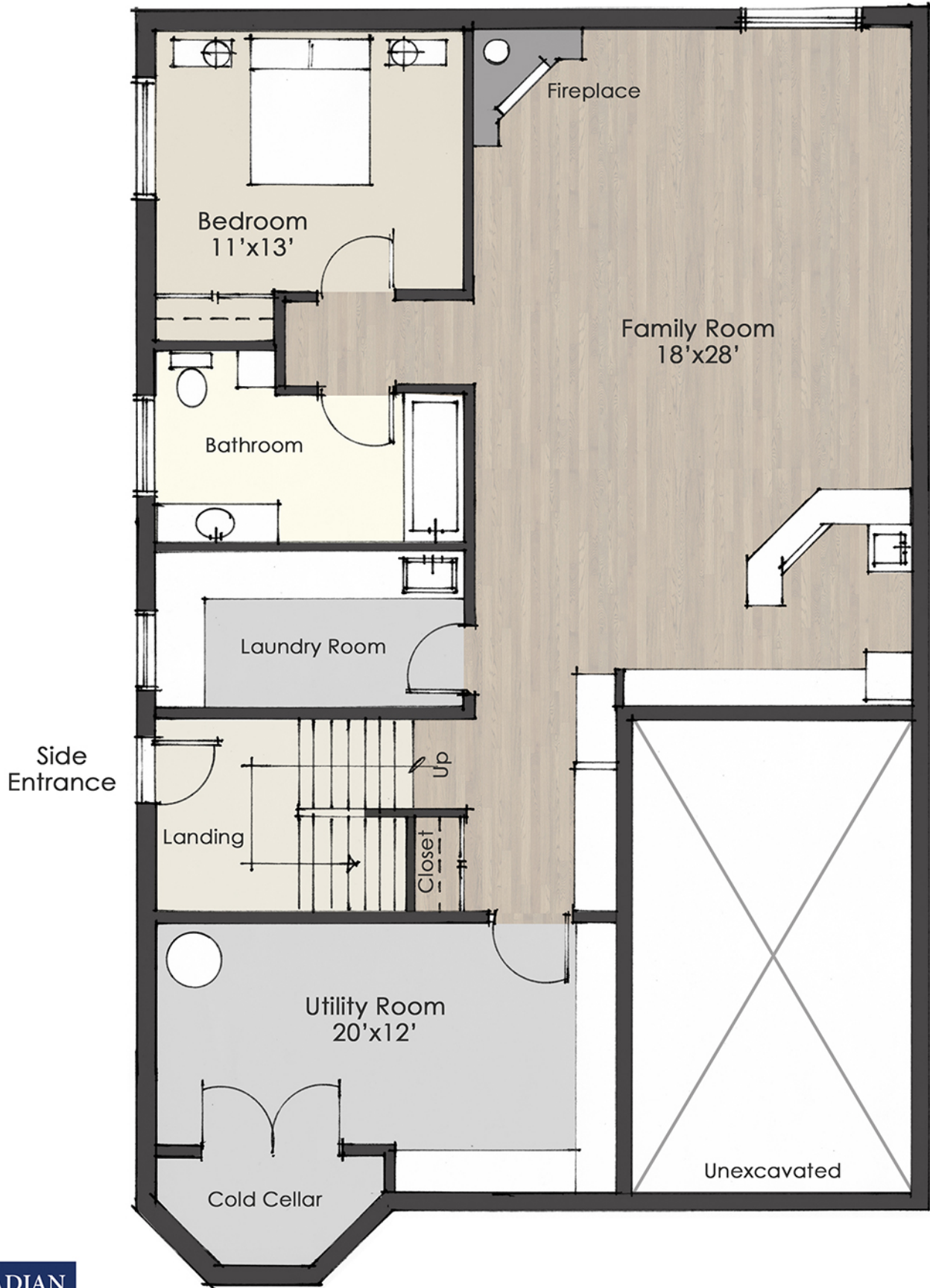
BASEMENT PLAN Freehold Unit #25 Richardson Lane
